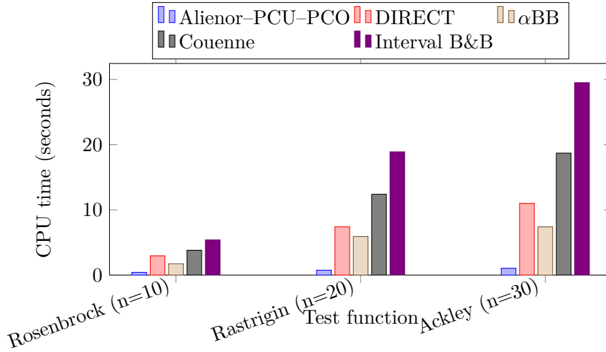
Fig. 1. Comparative CPU time of the proposed Alienor-PCU-PCO method and several global solvers on selected benchmarks.
